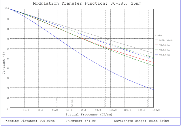
#36-385, 25mm FL f/4, Rugged Blue Series M12 Lens, Modulated Transfer Function (MTF) Plot, 400mm Working Distance, f4
