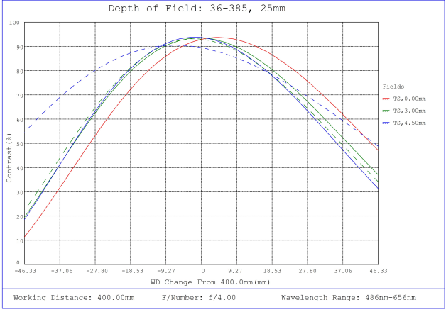
#36-385, 25mm FL f/4, Rugged Blue Series M12 Lens, Depth of Field Plot, 400mm Working Distance, f4
