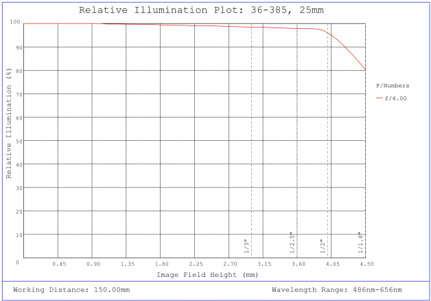
#36-385, 25mm FL f/4, Rugged Blue Series M12 Lens, Relative Illumination Plot
