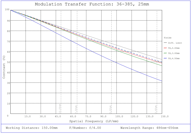
#36-385, 25mm FL f/4, Rugged Blue Series M12 Lens, Modulated Transfer Function (MTF) Plot, 150mm Working Distance, f4
