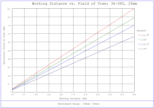
#36-385, 25mm FL f/4, Rugged Blue Series M12 Lens, Working Distance versus Field of View Plot
