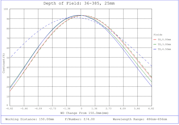
#36-385, 25mm FL f/4, Rugged Blue Series M12 Lens, Depth of Field Plot, 150mm Working Distance, f4
