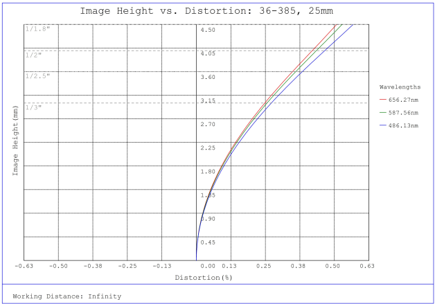
#36-385, 25mm FL f/4, Rugged Blue Series M12 Lens, Distortion Plot
