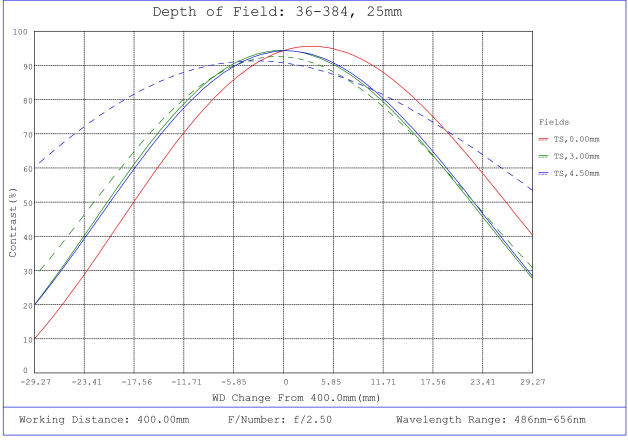
#36-384, 25mm FL f/2.5, Rugged Blue Series M12 Lens, Depth of Field Plot, 400mm Working Distance, f2.5
