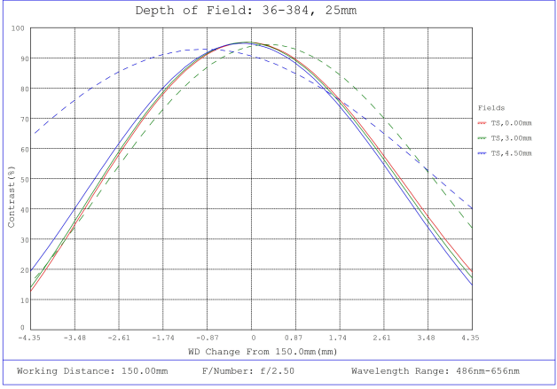
#36-384, 25mm FL f/2.5, Rugged Blue Series M12 Lens, Depth of Field Plot, 150mm Working Distance, f2.5
