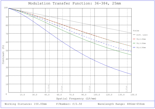
#36-384, 25mm FL f/2.5, Rugged Blue Series M12 Lens, Modulated Transfer Function (MTF) Plot, 150mm Working Distance, f2.5
