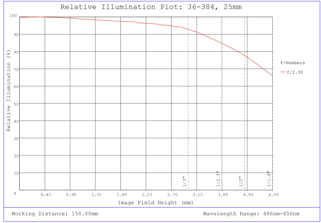
#36-384, 25mm FL f/2.5, Rugged Blue Series M12 Lens, Relative Illumination Plot
