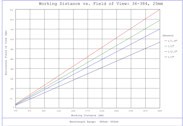
#36-384, 25mm FL f/2.5, Rugged Blue Series M12 Lens, Working Distance versus Field of View Plot
