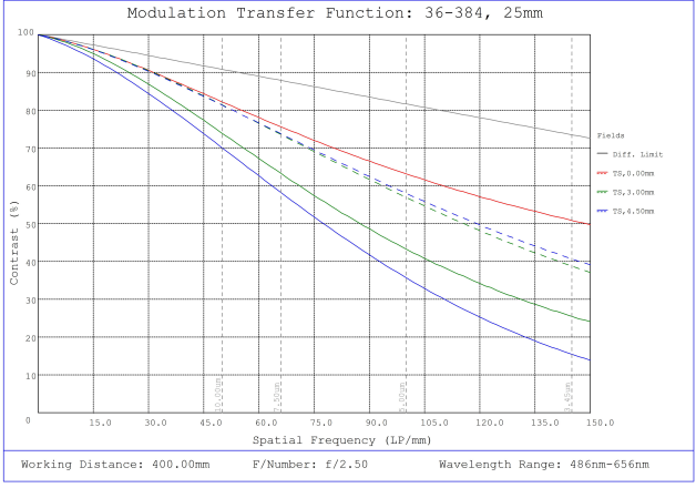
#36-384, 25mm FL f/2.5, Rugged Blue Series M12 Lens, Modulated Transfer Function (MTF) Plot, 400mm Working Distance, f2.5
