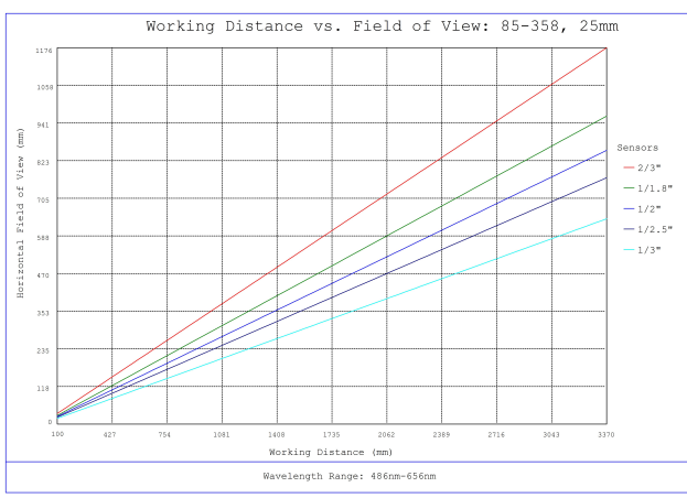
#85-358, 25mm, f/4 Ci Series Fixed Focal Length Lens, Working Distance versus Field of View Plot
