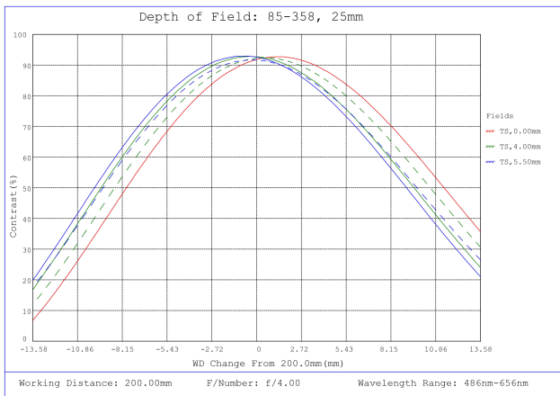
#85-358, 25mm, f/4 Ci Series Fixed Focal Length Lens, Depth of Field Plot, 200mm Working Distance, f4
