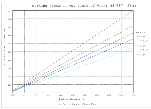
#85-357, 25mm, f/2.8 Ci Series Fixed Focal Length Lens, Working Distance versus Field of View Plot
