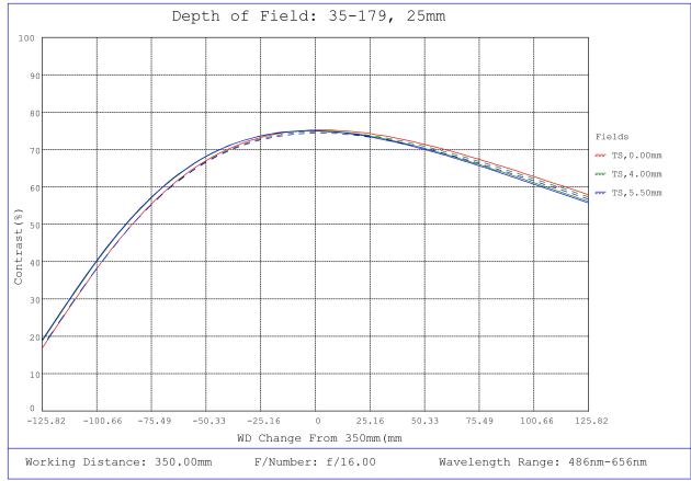
#35-179, 25mm, f/16 Cr Series Fixed Focal Length Lens, Depth of Field Plot, 350mm Working Distance, f16
