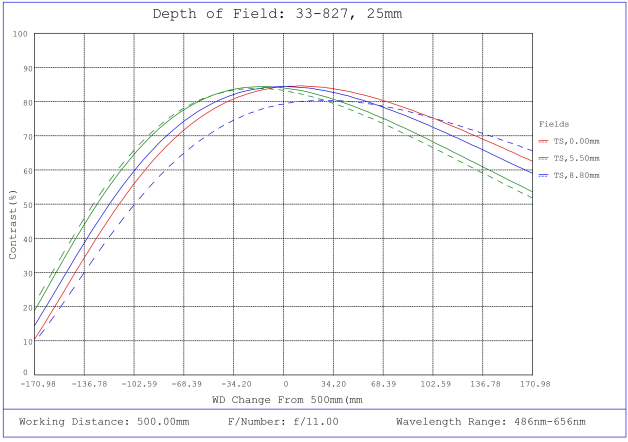
#33-827, 25mm f/11.0, HPi Series Fixed Focal Length Lens, Depth of Field Plot, 500mm Working Distance, f11
