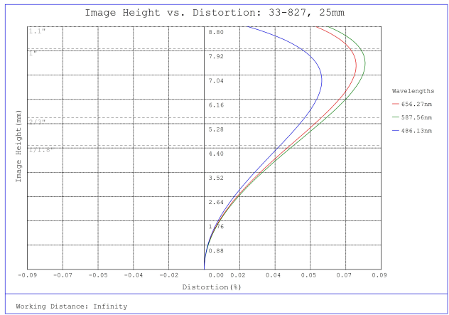
#33-827, 25mm f/11.0, HPi Series Fixed Focal Length Lens, Distortion Plot
