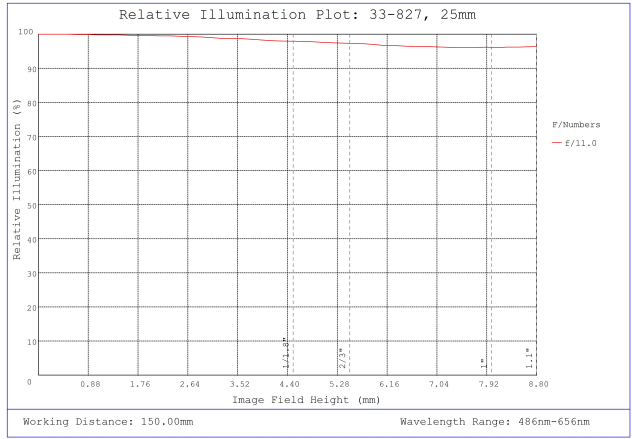
#33-827, 25mm f/11.0, HPi Series Fixed Focal Length Lens, Relative Illumination Plot
