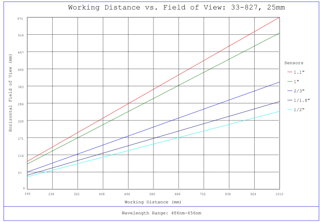
#33-827, 25mm f/11.0, HPi Series Fixed Focal Length Lens, Working Distance versus Field of View Plot
