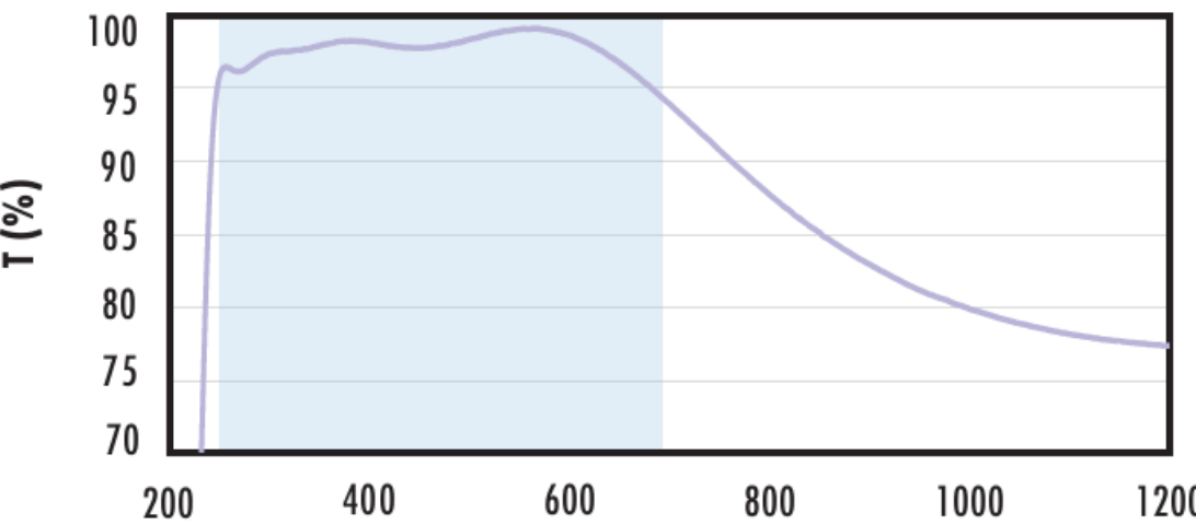
Fused Silica with UV-VIS Coating Typical Transmission
