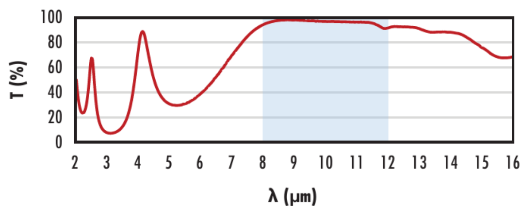
8-12 \mu m AR Coated Germanium Typical Transmission
