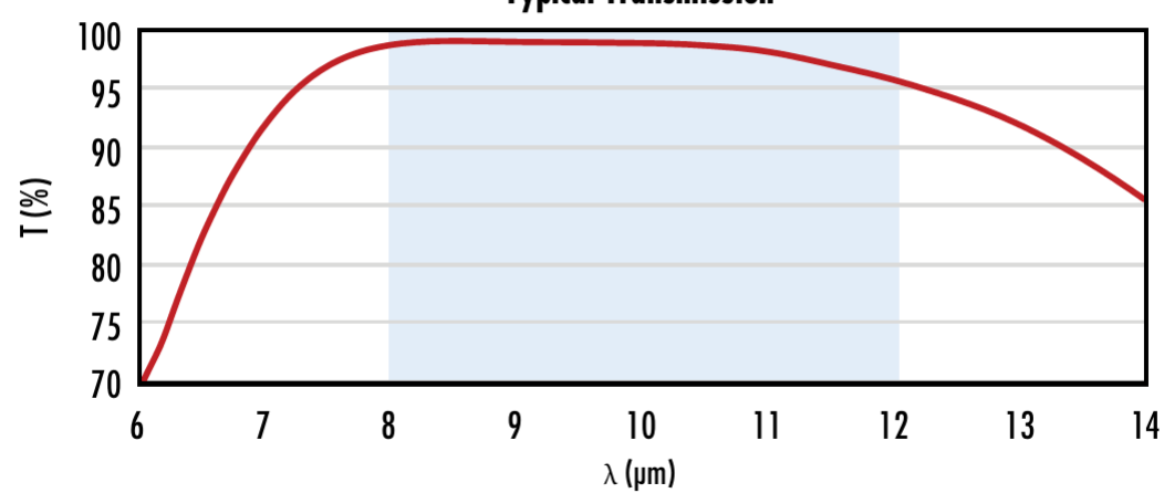
ZnSe with 8-12μm AR Coating Typical Transmission
