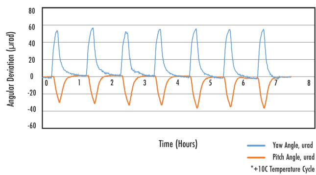
EO #28-747 Pitch and Yaw During Thermal Cycling
