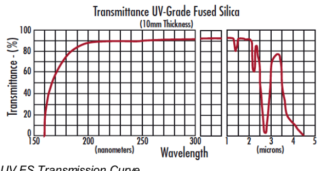
UV FS Transmission Curve
