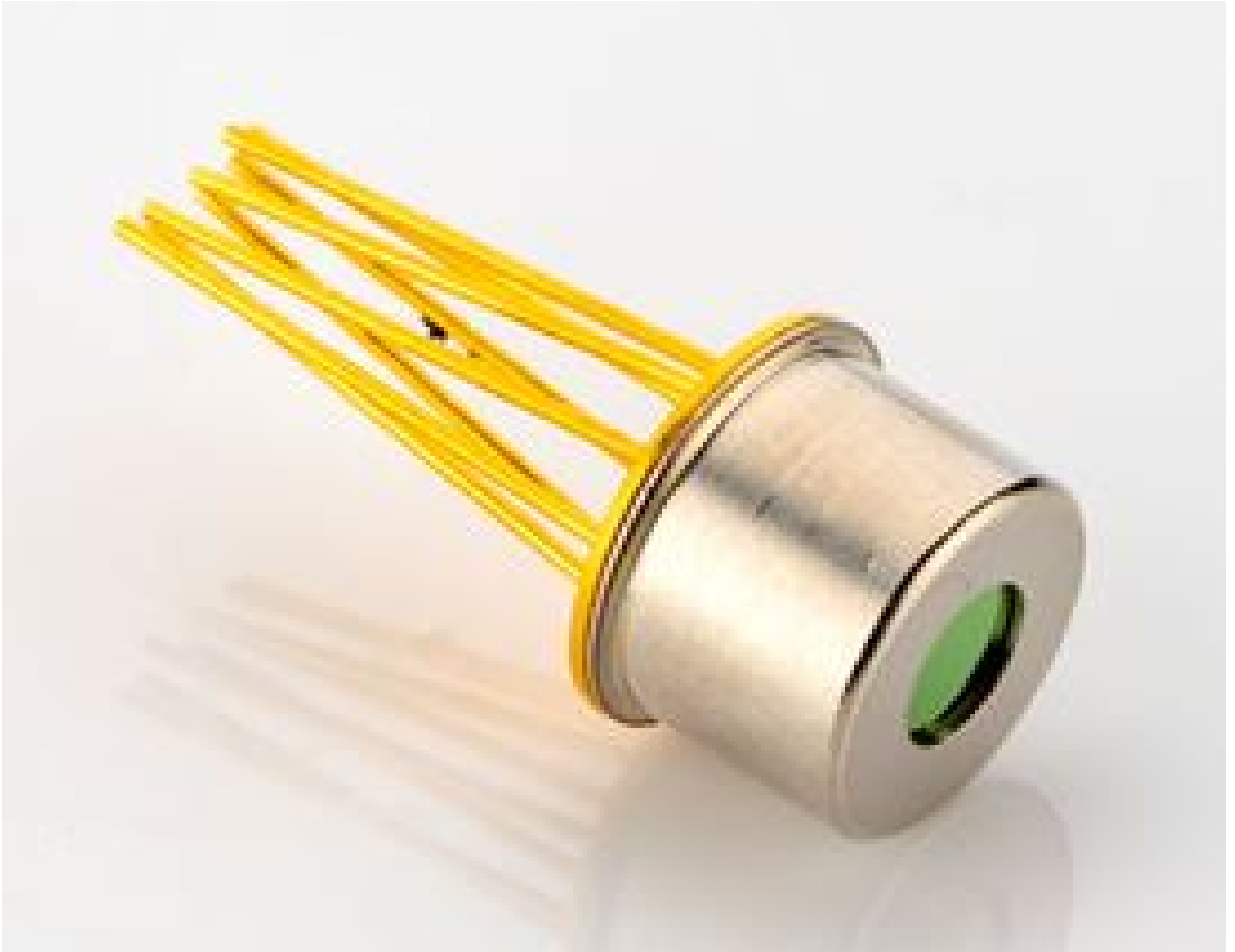
2 - 5.5um InAsSb Photovoltaic Multi-Juncton IR Detector, PVMA-1TE-5-1x1-TO39-pSiAR-70
