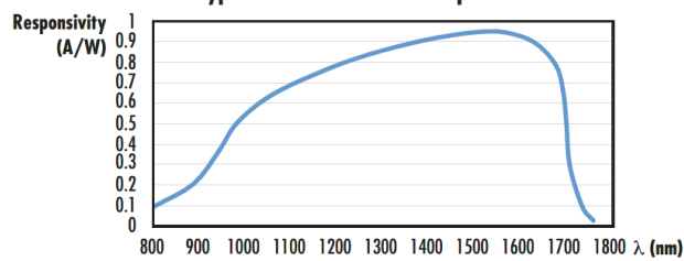
Typical InGaAs Detector Response Curve
