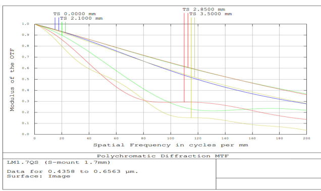
1.7mm FL, f/4, Low Distortion M12 Lens, MTF Plot
