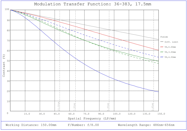
#36-383, 17.5mm FL f/8, Rugged Blue Series M12 Lens, Modulated Transfer Function (MTF) Plot, 150mm Working Distance, f8
