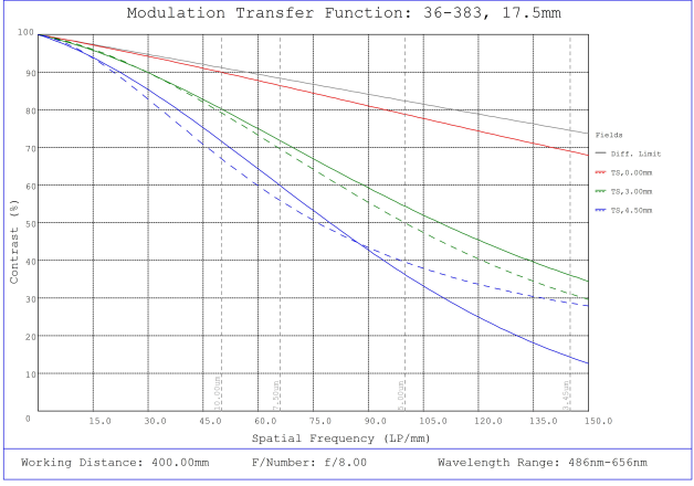
#36-383, 17.5mm FL f/8, Rugged Blue Series M12 Lens, Modulated Transfer Function (MTF) Plot, 400mm Working Distance, f8
