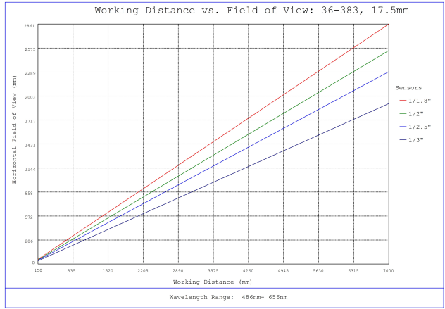
#36-383, 17.5mm FL f/8, Rugged Blue Series M12 Lens, Working Distance versus Field of View Plot
