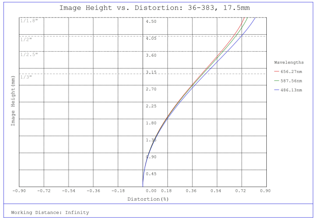
#36-383, 17.5mm FL f/8, Rugged Blue Series M12 Lens, Distortion Plot
