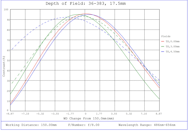
#36-383, 17.5mm FL f/8, Rugged Blue Series M12 Lens, Depth of Field Plot, 150mm Working Distance, f8
