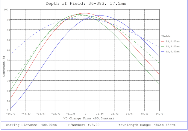
#36-383, 17.5mm FL f/8, Rugged Blue Series M12 Lens, Depth of Field Plot, 400mm Working Distance, f8
