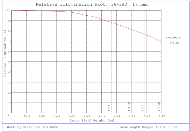
#36-383, 17.5mm FL f/8, Rugged Blue Series M12 Lens, Relative Illumination Plot
