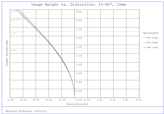
#33-887, 16mm, f/8 UCi Series Fixed Focal Length Lens, Distortion Plot
