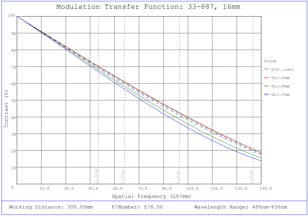
#33-887, 16mm, f/8 UCi Series Fixed Focal Length Lens, Modulated Transfer Function (MTF) Plot, 300mm Working Distance, f8
