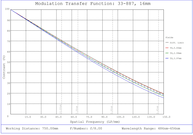
#33-887, 16mm, f/8 UCi Series Fixed Focal Length Lens, Modulated Transfer Function (MTF) Plot, 750mm Working Distance, f8
