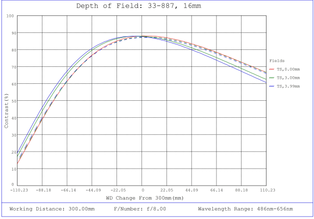
#33-887, 16mm, f/8 UCi Series Fixed Focal Length Lens, Depth of Field Plot, 300mm Working Distance, f8
