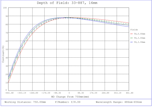
#33-887, 16mm, f/8 UCi Series Fixed Focal Length Lens, Depth of Field Plot, 750mm Working Distance, f8
