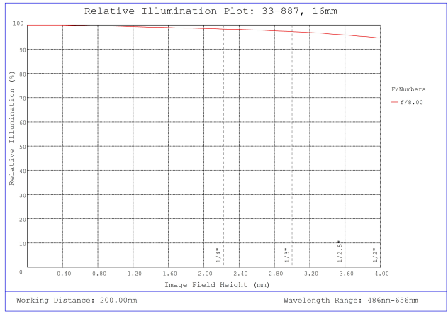
#33-887, 16mm, f/8 UCi Series Fixed Focal Length Lens, Relative Illumination Plot
