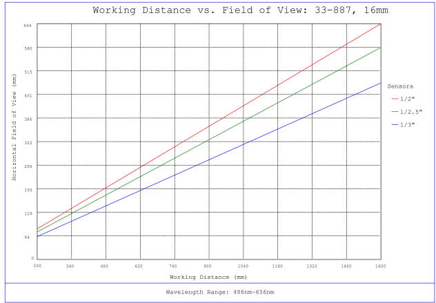
#33-887, 16mm, f/8 UCi Series Fixed Focal Length Lens, Working Distance versus Field of View Plot
