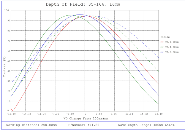
#35-164, 16mm, f/1.8 Cr Series Fixed Focal Length Lens, Depth of Field Plot, 200mm Working Distance, f1.8
