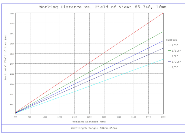
#85-348, 16mm, f/1.6 Ci Series Fixed Focal Length Lens, Working Distance versus Field of View Plot
