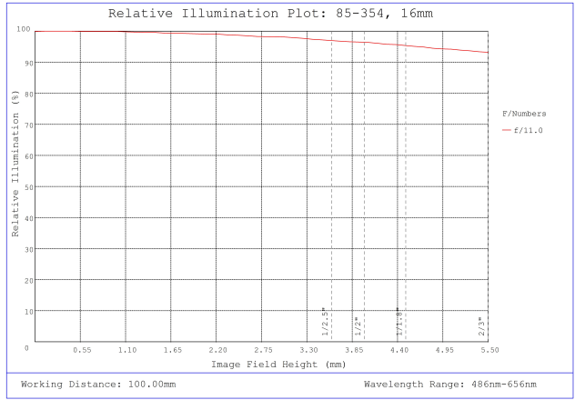
#85-354, 16mm, f/11 Ci Series Fixed Focal Length Lens, Relative Illumination Plot
