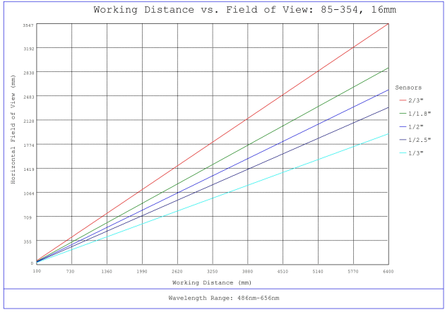
#85-354, 16mm, f/11 Ci Series Fixed Focal Length Lens, Working Distance versus Field of View Plot
