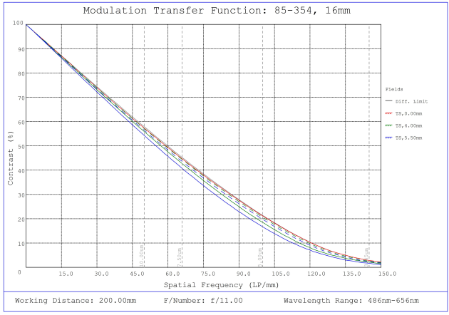
#85-354, 16mm, f/11 Ci Series Fixed Focal Length Lens, Modulated Transfer Function (MTF) Plot, 200mm Working Distance, f11
