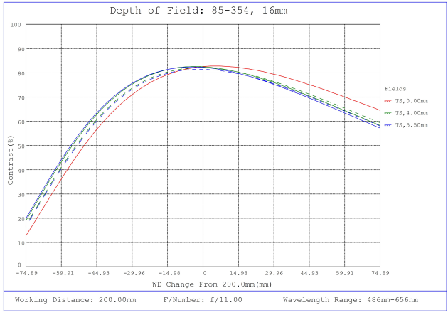
#85-354, 16mm, f/11 Ci Series Fixed Focal Length Lens, Depth of Field Plot, 200mm Working Distance, f11
