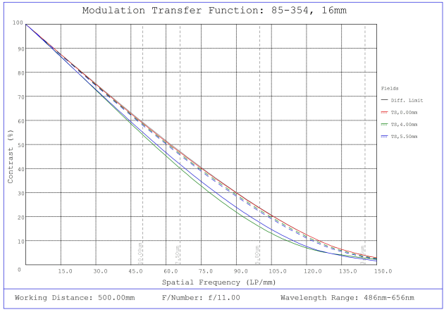
#85-354, 16mm, f/11 Ci Series Fixed Focal Length Lens, Modulated Transfer Function (MTF) Plot, 500mm Working Distance, f11
