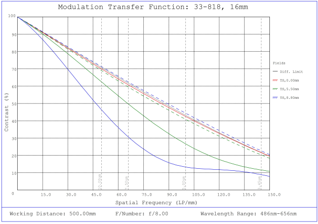
#33-818, 16mm f/8, HPI Series Fixed Focal Length Lens, Modulated Transfer Function (MTF) Plot, 500mm Working Distance, f8
