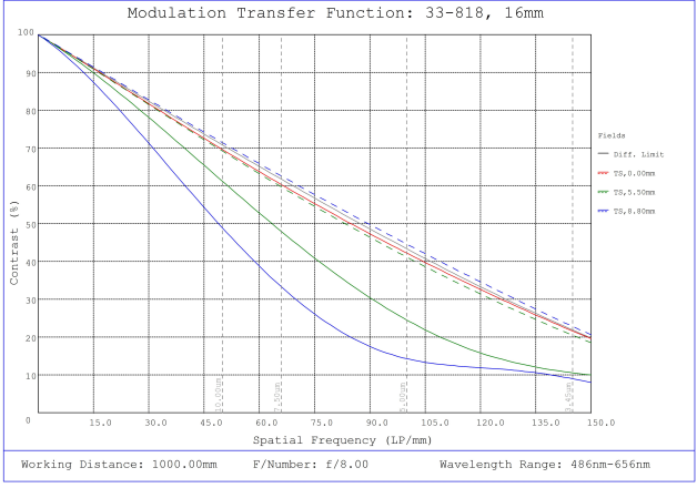
#33-818, 16mm f/8, HPI Series Fixed Focal Length Lens, Modulated Transfer Function (MTF) Plot, 1000mm Working Distance, f8
