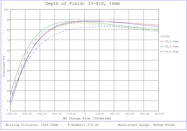
#33-818, 16mm f/8, HPI Series Fixed Focal Length Lens, Depth of Field Plot, 1000mm Working Distance, f8
