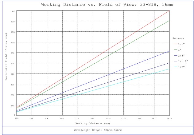
#33-818, 16mm f/8, HPI Series Fixed Focal Length Lens, Working Distance versus Field of View Plot
