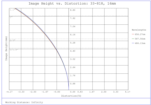
#33-818, 16mm f/8, HPI Series Fixed Focal Length Lens, Distortion Plot
