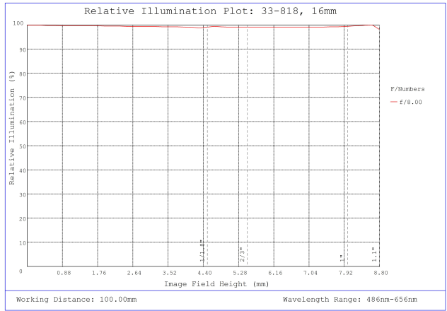
#33-818, 16mm f/8, HPI Series Fixed Focal Length Lens, Relative Illumination Plot
