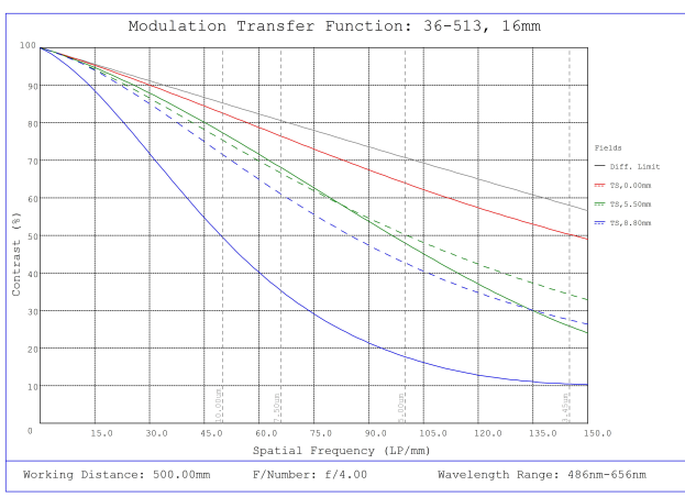
#36-513, 16mm f/4, HPr Series Fixed Focal Length Lens, Modulated Transfer Function (MTF) Plot, 500mm Working Distance, f4
