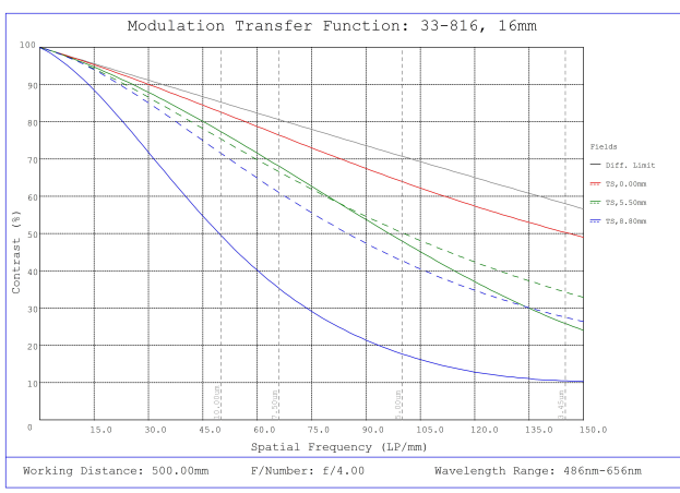
#33-816, 16mm f/4, HPI Series Fixed Focal Length Lens, Modulated Transfer Function (MTF) Plot, 500mm Working Distance, f4
