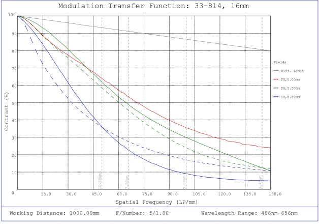
#33-814, 16mm f/1.8, HPi Series Fixed Focal Length Lens, Modulated Transfer Function (MTF) Plot, 1000mm Working Distance, f1.8
