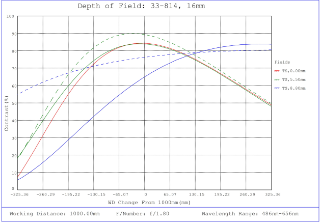
#33-814, 16mm f/1.8, HPi Series Fixed Focal Length Lens, Depth of Field Plot, 1000mm Working Distance, f1.8
