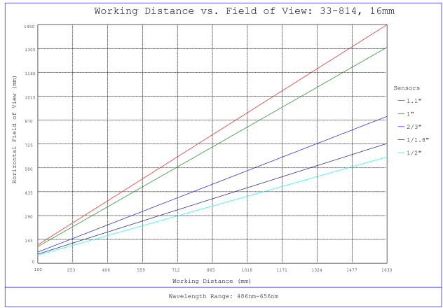
#33-814, 16mm f/1.8, HPI Series Fixed Focal Length Lens, Working Distance versus Field of View Plot
