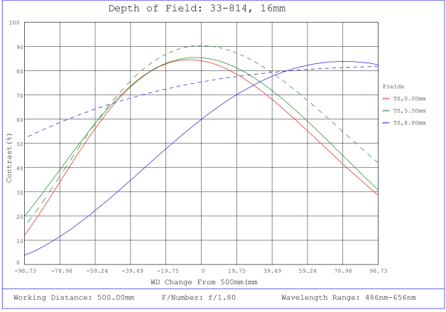
#33-814, 16mm f/1.8, HPi Series Fixed Focal Length Lens, Depth of Field Plot, 500mm Working Distance, f1.8
