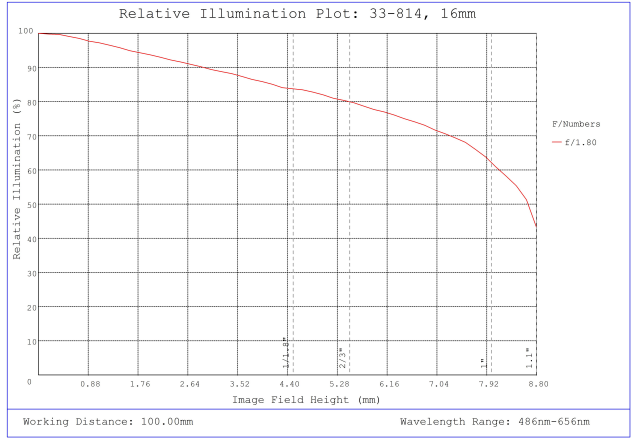
#33-814, 16mm f/1.8, HPI Series Fixed Focal Length Lens, Relative Illumination Plot
