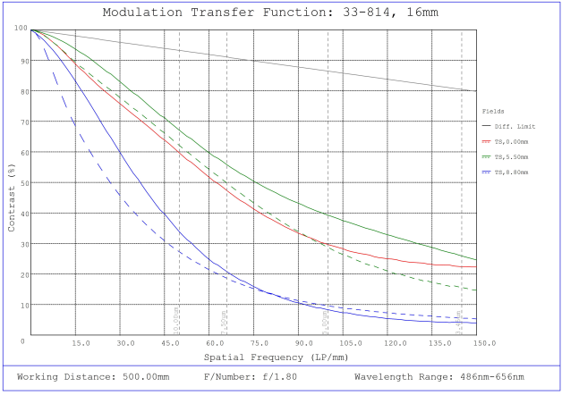
#33-814, 16mm f/1.8, HPi Series Fixed Focal Length Lens, Modulated Transfer Function (MTF) Plot, 500mm Working Distance, f1.8
