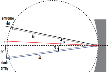
Polychromator Configuration
