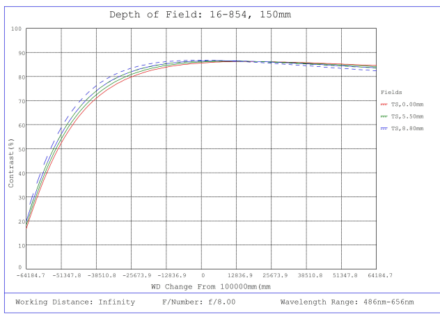
#16-854, 150mm, f/8 Athermal Lens, Depth of Field Plot, 10000mm Working Distance, f8
