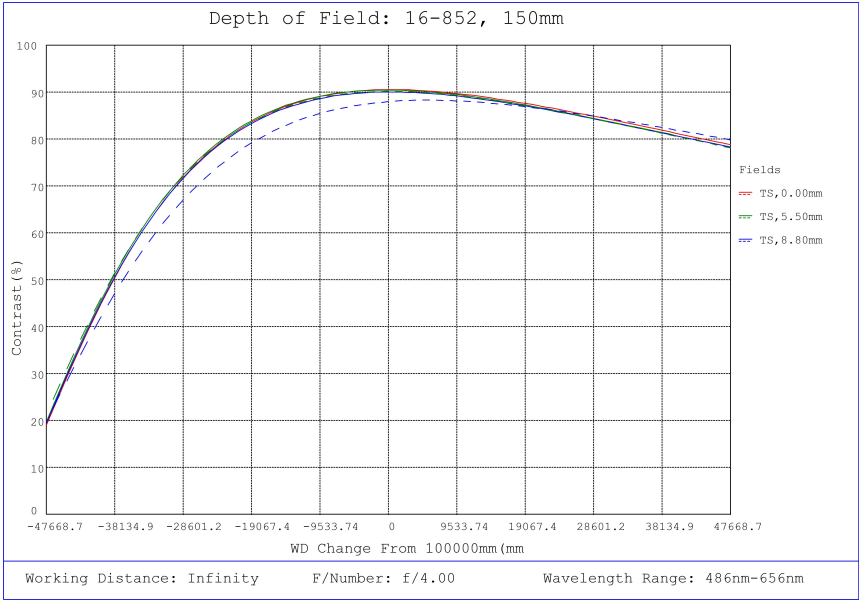
#16-852, 150mm, f/4 Athermal Lens, Depth of Field Plot, 10000mm Working Distance, f4
