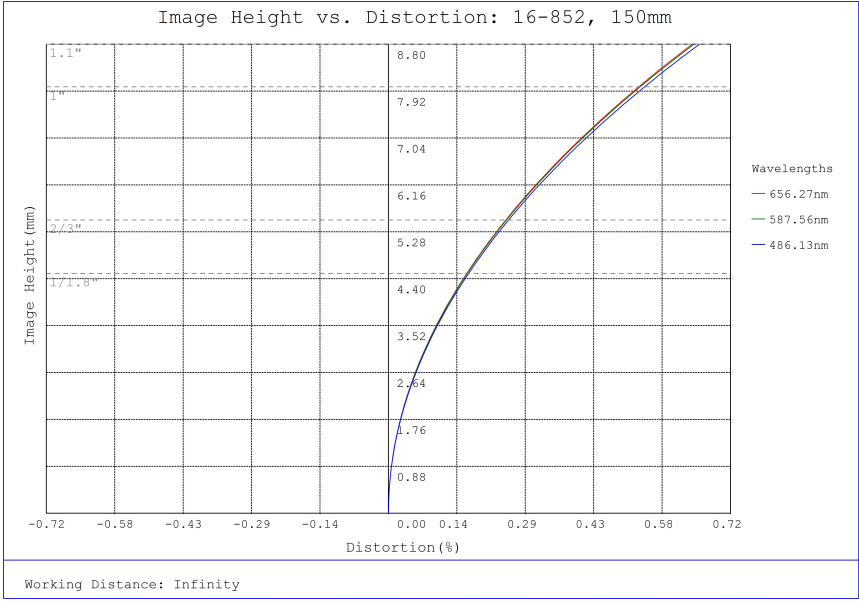
#16-852, 150mm, f/4 Athermal Lens, Distortion Plot
