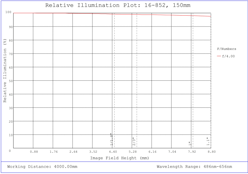
#16-852, 150mm, f/4 Athermal Lens, Relative Illumination Plot
