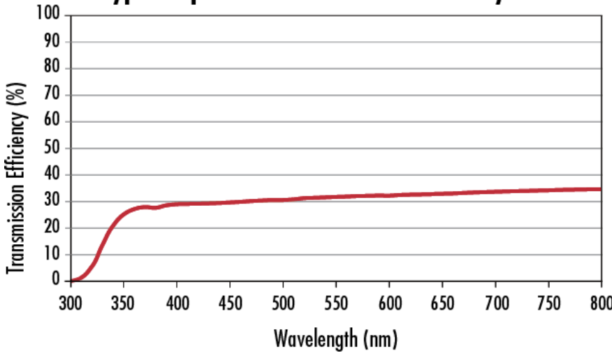
Typical Spectral Transmission Efficiency Curve
