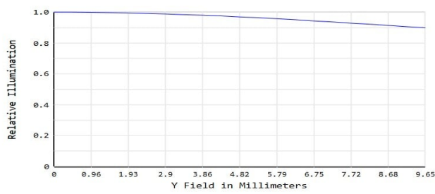
#22-835 - 12mm Focal Length, UAV Series Fixed Focal Length Lens, Relative Illumination Plot
