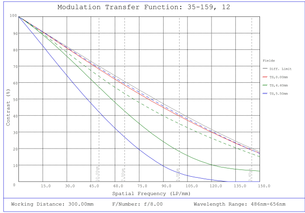
#35-159, 12mm, f/8 Cr Series Fixed Focal Length Lens, Modulated Transfer Function (MTF) Plot, 300mm Working Distance, f8
