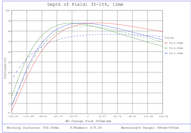
#35-159, 12mm, f/8 Cr Series Fixed Focal Length Lens, Depth of Field Plot, 300mm Working Distance, f8
