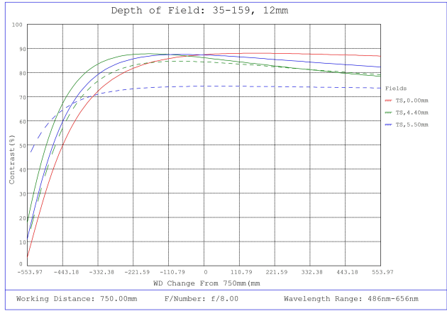
#35-159, 12mm, f/8 Cr Series Fixed Focal Length Lens, Depth of Field Plot, 750mm Working Distance, f8
