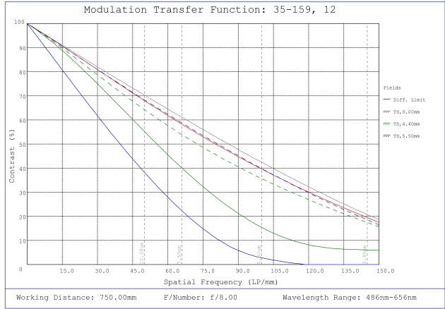
#35-159, 12mm, f/8 Cr Series Fixed Focal Length Lens, Modulated Transfer Function (MTF) Plot, 750mm Working Distance, f8
