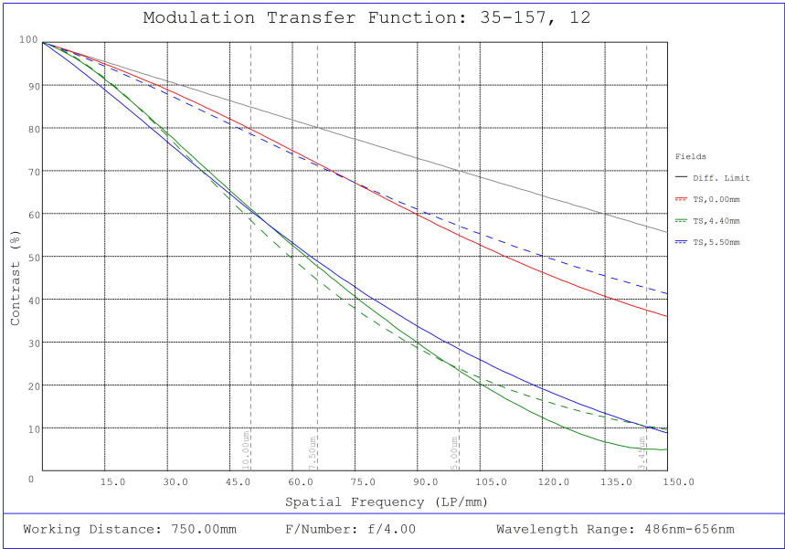
#35-157, 12mm, f/4 Cr Series Fixed Focal Length Lens, Modulated Transfer Function (MTF) Plot, 750mm Working Distance, f4
