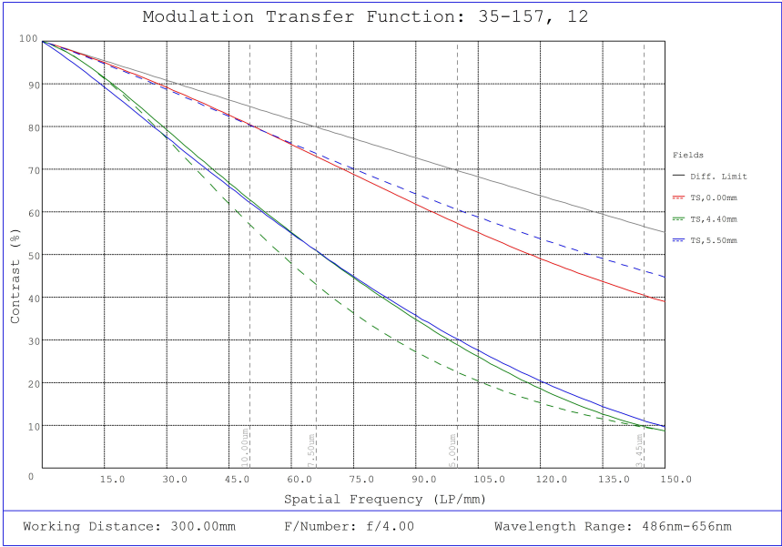
#35-157, 12mm, f/4 Cr Series Fixed Focal Length Lens, Modulated Transfer Function (MTF) Plot, 300mm Working Distance, f4
