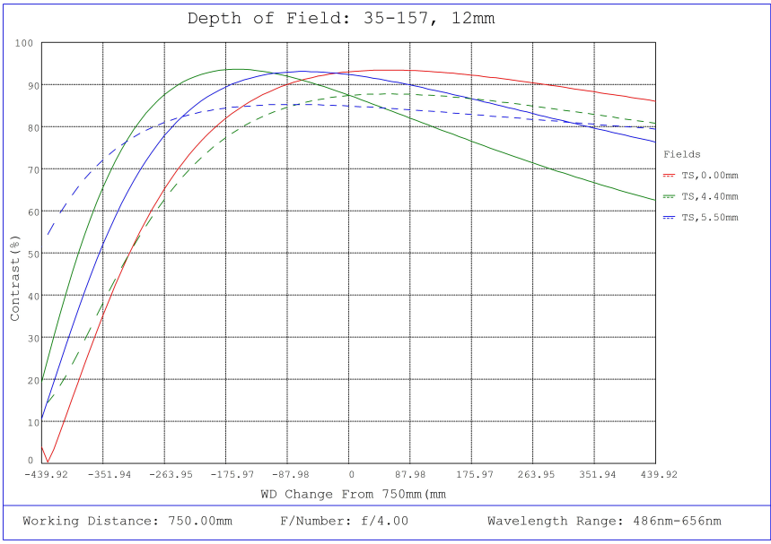
#35-157, 12mm, f/4 Cr Series Fixed Focal Length Lens, Depth of Field Plot, 750mm Working Distance, f4
