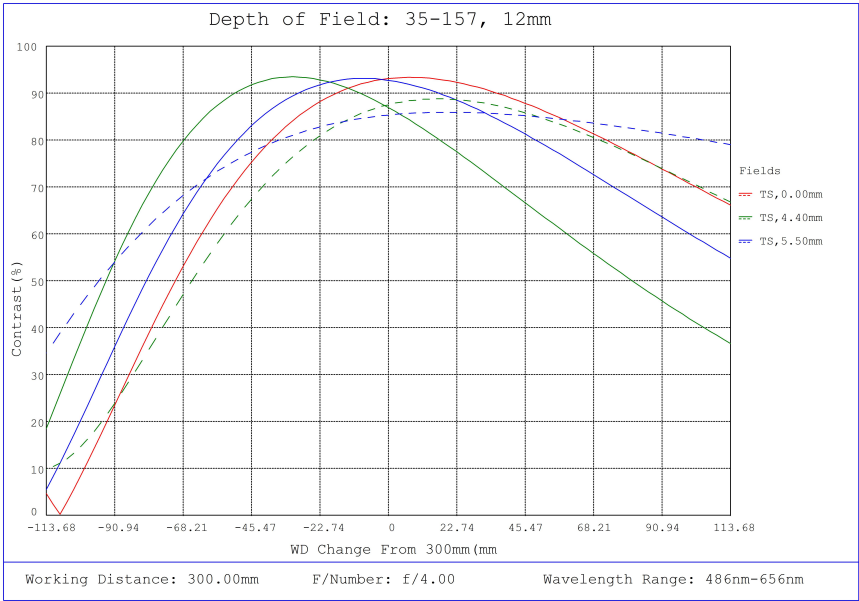
#35-157, 12mm, f/4 Cr Series Fixed Focal Length Lens, Depth of Field Plot, 300mm Working Distance, f4
