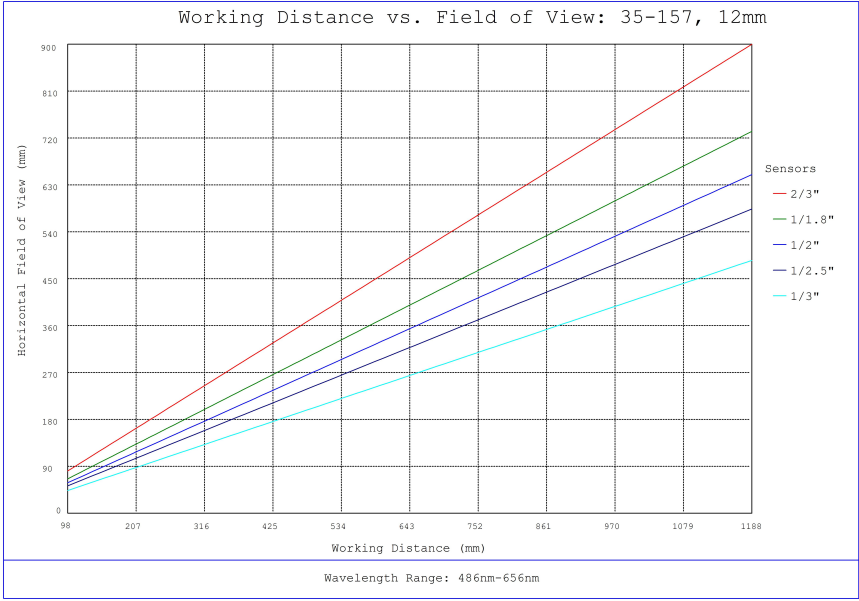
#35-157, 12mm, f/4 Cr Series Fixed Focal Length Lens, Working Distance versus Field of View Plot
