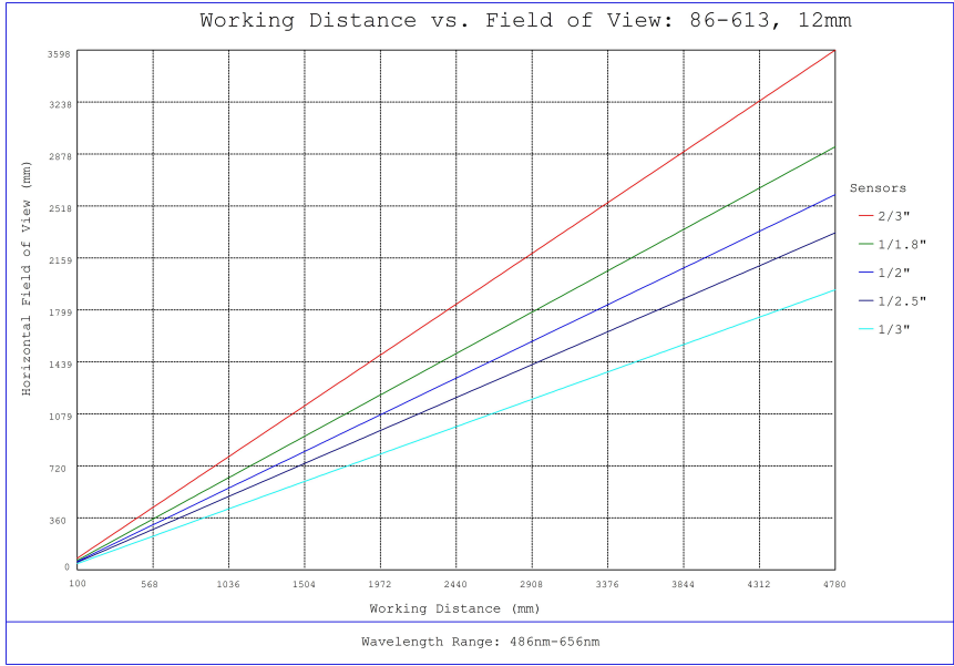
#86-613, 12mm, f/16 Ci Series Fixed Focal Length Lens, Working Distance versus Field of View Plot
