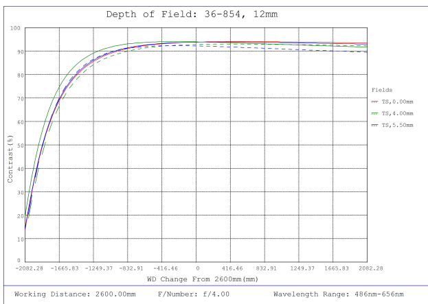
#36-854, 12mm f/4, 1000mm-∞ Primary WD, HRr Series Fixed Focal Length Lens, Depth of Field Plot, 2600mm Working Distance, f4
