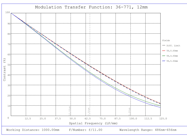
#36-771, 12mm f/11, 1000mm-∞ Primary WD, HRi Series Fixed Focal Length Lens, Modulated Transfer Function (MTF) Plot, 1000mm Working Distance, f11
