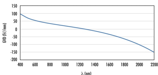
Calculated GVD of Fused Silica
