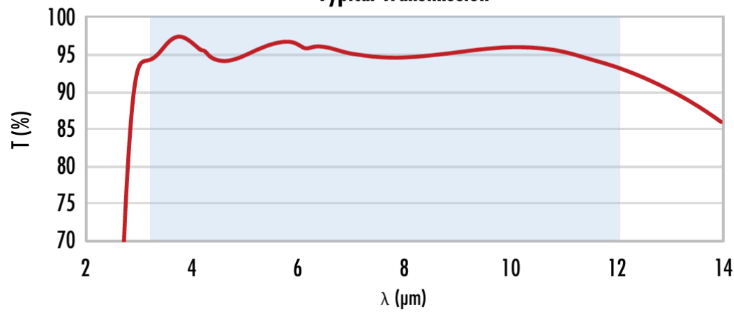
ZnSe with 3-12um AR Coating Typical Transmission
