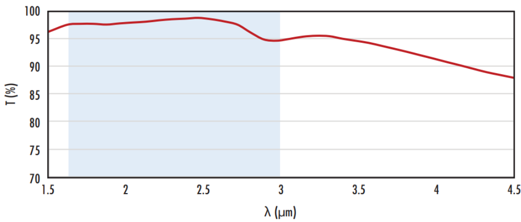
ZnSe with 1.65-3um AR Coating Typical Transmission
