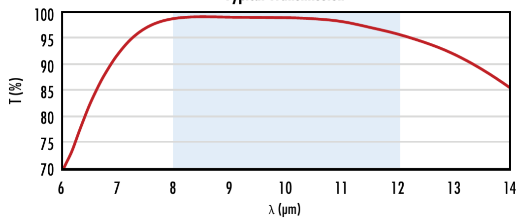
ZnSe with 8-12um AR Coating Typical Transmission
