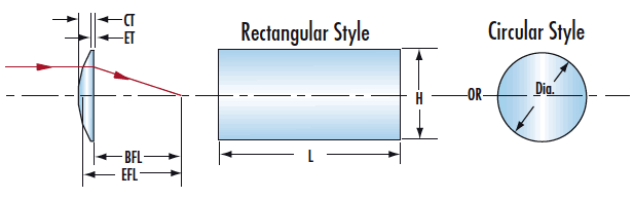
Circular And Rectangular Cylinder Lenses
