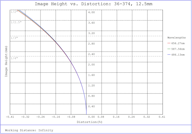
#36-374, 12.5mm FL f/5.6, Rugged Blue Series M12 Lens, Distortion Plot
