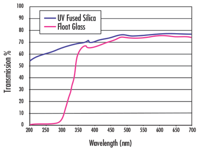
Diffuser Transmission
