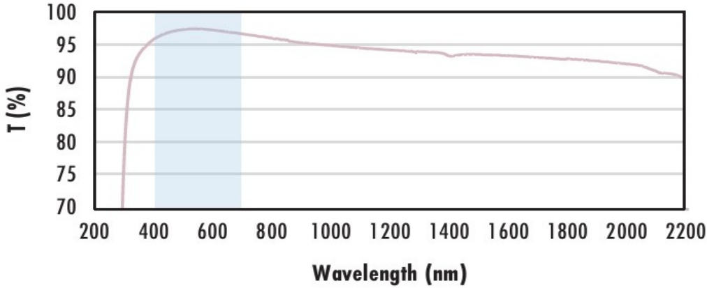
N-BK7 with VIS-EXT Coating Typical Transmission
