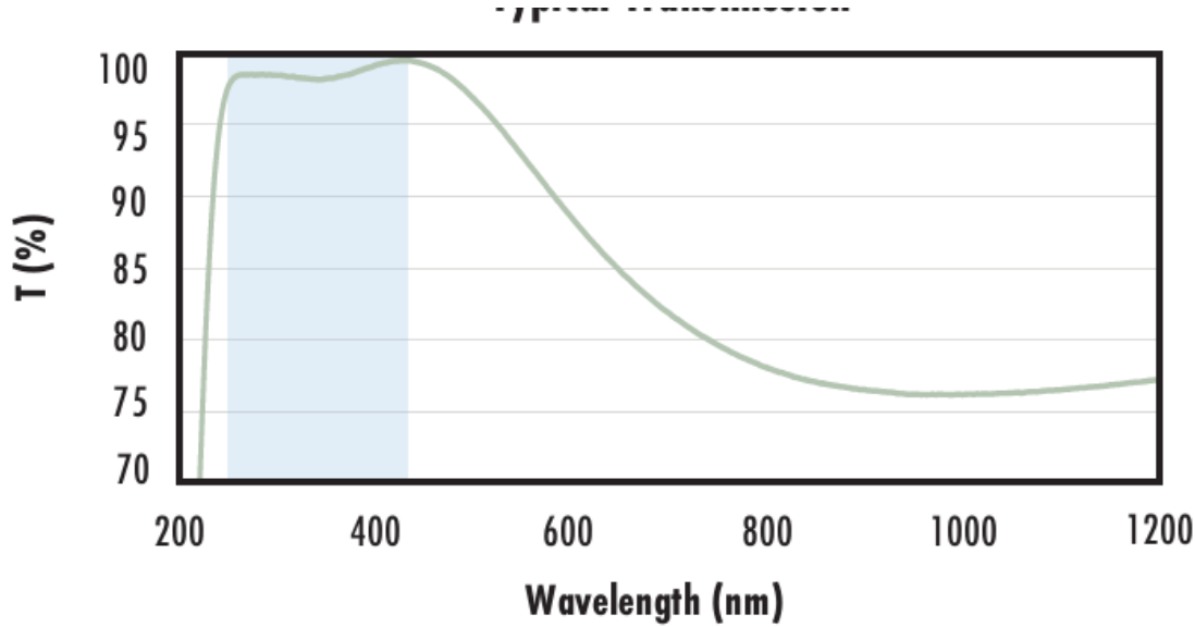
Fused Silica with UV-VIS Coating Typical Transmission
