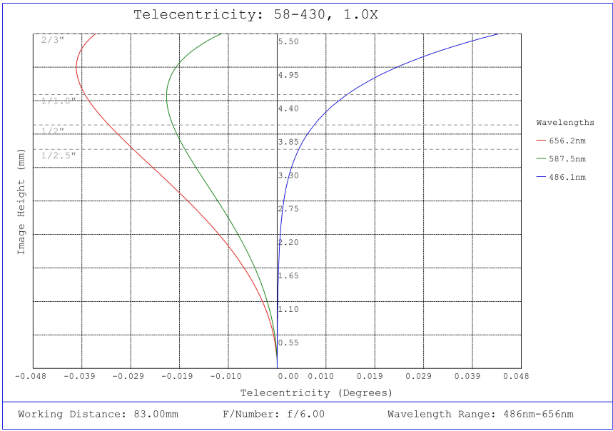
#58-430, 1.0X SilverTL™ Telecentric Lens, Telecentricity Plot
