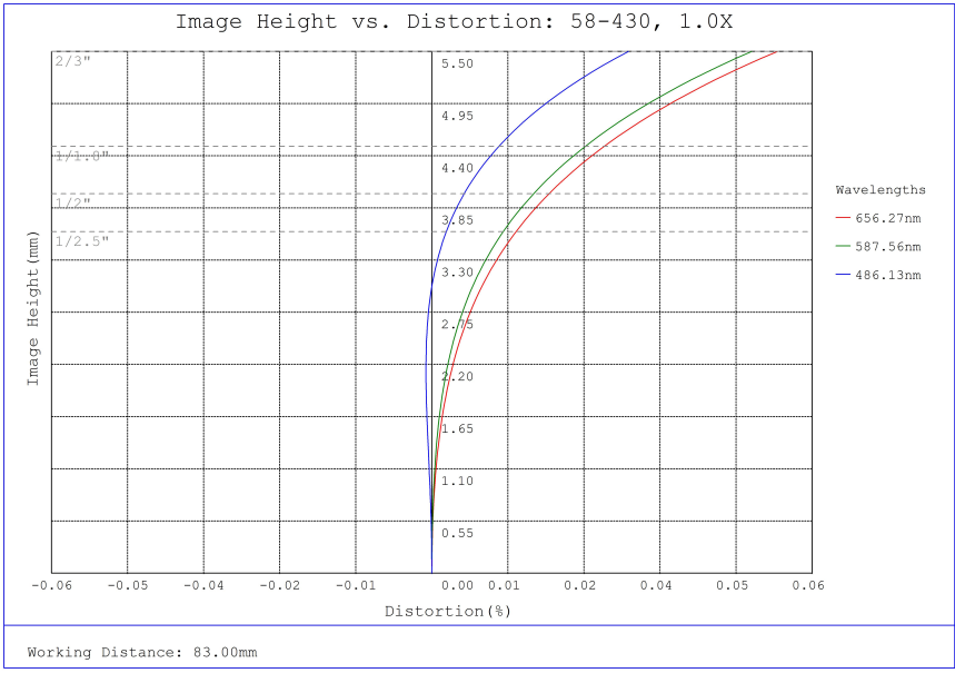
#58-430, 1.0X SilverTL™ Telecentric Lens, Distortion Plot
