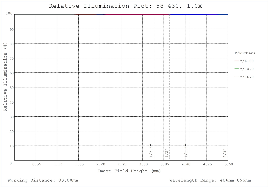
#58-430, 1.0X SilverTL™ Telecentric Lens, Relative Illumination Plot
