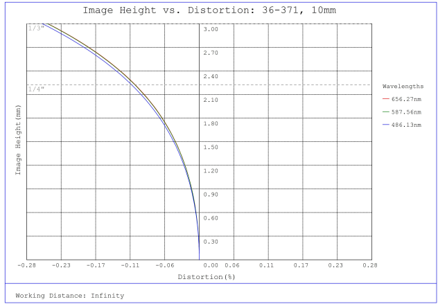
#36-371, 10mm FL f/8, Rugged Blue Series M12 Lens, Distortion Plot
