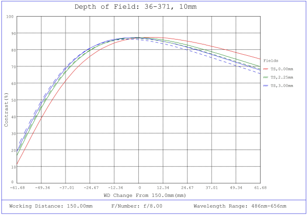
#36-371, 10mm FL f/8, Rugged Blue Series M12 Lens, Depth of Field Plot, 150mm Working Distance, f8
