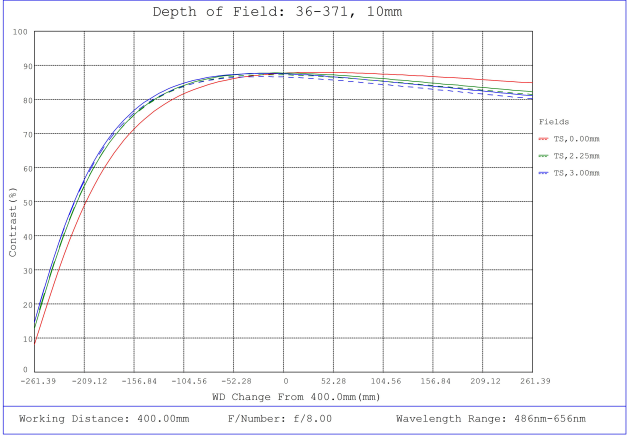
#36-371, 10mm FL f/8, Rugged Blue Series M12 Lens, Depth of Field Plot, 400mm Working Distance, f8
