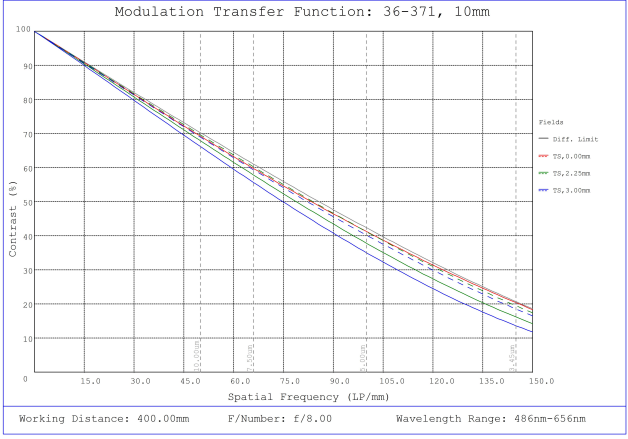
#36-371, 10mm FL f/8, Rugged Blue Series M12 Lens, Modulated Transfer Function (MTF) Plot, 400mm Working Distance, f8
