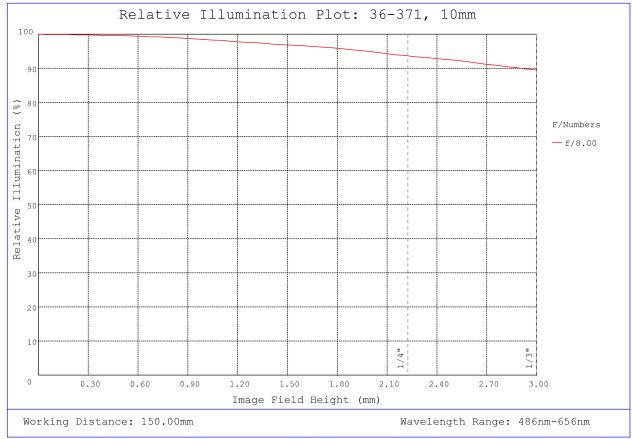
#36-371, 10mm FL f/8, Rugged Blue Series M12 Lens, Relative Illumination Plot
