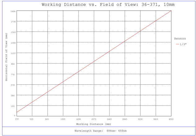
#36-371, 10mm FL f/8, Rugged Blue Series M12 Lens, Working Distance versus Field of View Plot
