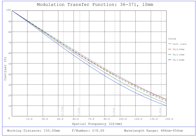
#36-371, 10mm FL f/8, Rugged Blue Series M12 Lens, Modulated Transfer Function (MTF) Plot, 150mm Working Distance, f8
