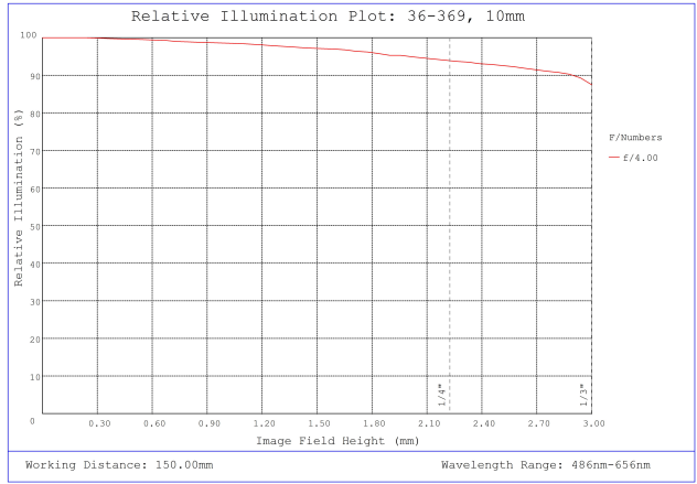
#36-369, 10mm FL f/4, Rugged Blue Series M12 Lens, Relative Illumination Plot
