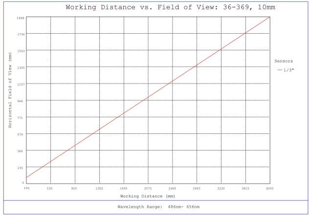
#36-369, 10mm FL f/4, Rugged Blue Series M12 Lens, Working Distance versus Field of View Plot
