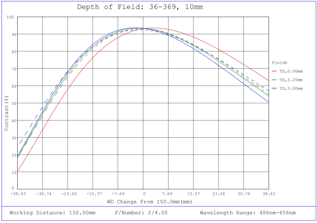
#36-369, 10mm FL f/4, Rugged Blue Series M12 Lens, Depth of Field Plot, 150mm Working Distance, f4
