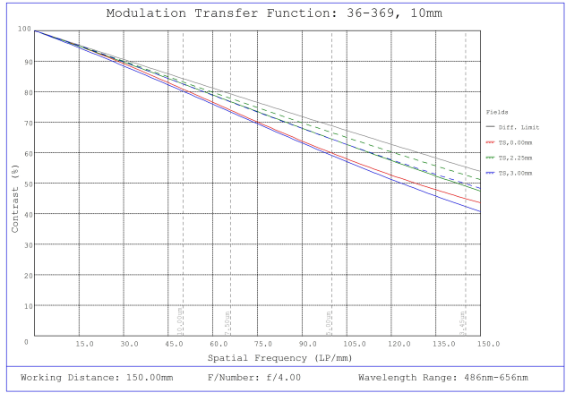
#36-369, 10mm FL f/4, Rugged Blue Series M12 Lens, Modulated Transfer Function (MTF) Plot, 150mm Working Distance, f4
