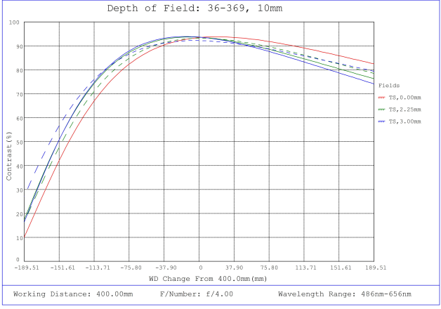
#36-369, 10mm FL f/4, Rugged Blue Series M12 Lens, Depth of Field Plot, 400mm Working Distance, f4
