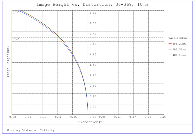
#36-369, 10mm FL f/4, Rugged Blue Series M12 Lens, Distortion Plot
