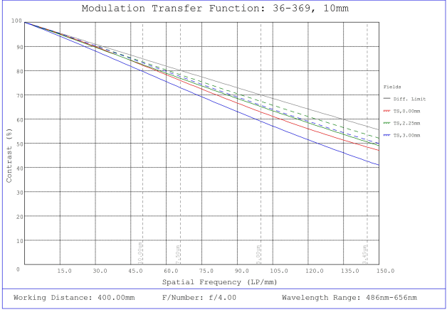
#36-369, 10mm FL f/4, Rugged Blue Series M12 Lens, Modulated Transfer Function (MTF) Plot, 400mm Working Distance, f4
