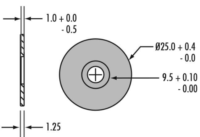
Mounted Precision Air Slits
