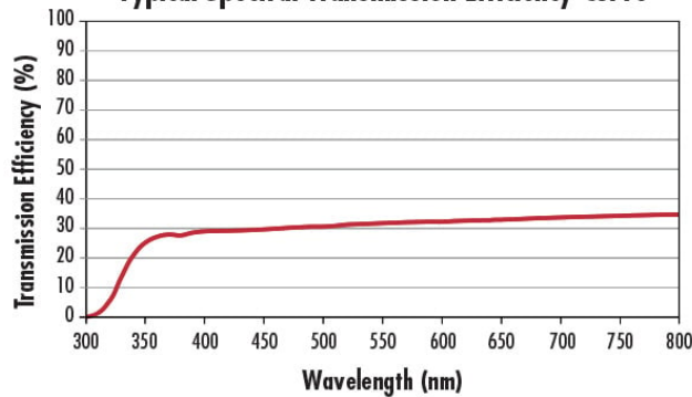
Typical Spectral Transmission Efficiency Curve
