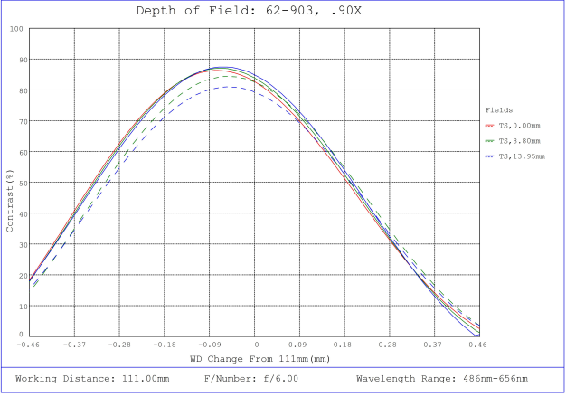
#62-903, 0.9X, 28.7mm M42 x 1.0 (6.56mm) PlatinumTL™ Telecentric Lens, Depth of Field Plot, 111mm Working Distance, f6
