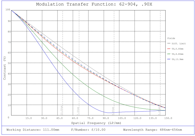
#62-904, 0.9X, 28.7mm M42 x 1.0 (19.53mm) PlatinumTL™ Telecentric Lens, Modulated Transfer Function (MTF) Plot, 111mm Working Distance, f10
