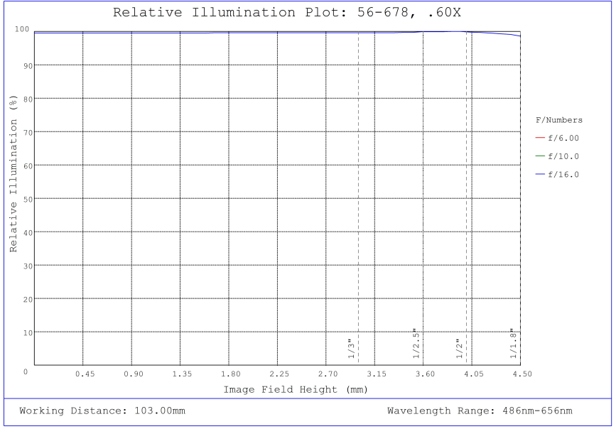
#56-678, 0.60X SilverTL™ Telecentric Lens, Relative Illumination Plot
