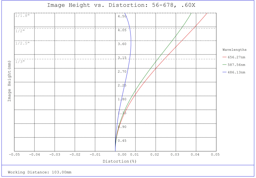
#56-678, 0.60X SilverTL™ Telecentric Lens, Distortion Plot
