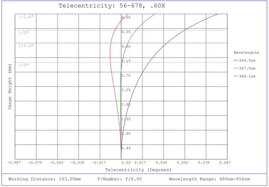
#56-678, 0.60X SilverTL™ Telecentric Lens, Telecentricity Plot
