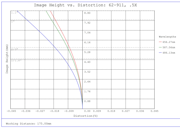
#62-911, 0.5X CobaltTL Telecentric Lens, Distortion Plot
