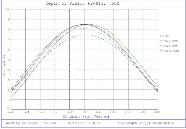
#62-913, 0.5X, 28.7mm M42 x 1.0 (6.56mm) PlatinumTL™ Telecentric Lens, Depth of Field Plot, 175mm Working Distance, f10
