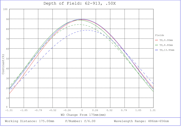
#62-913, 0.5X, 28.7mm M42 x 1.0 (6.56mm) PlatinumTL™ Telecentric Lens, Depth of Field Plot, 175mm Working Distance, f6
